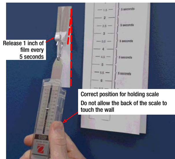
FIGURE 5 Release Test
